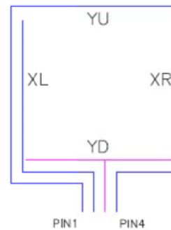
TOUCH PANEL PIN ASSIGNMENT
