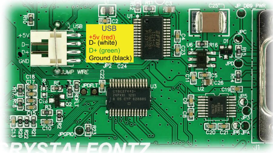
Figure 11. USB Connector Pins Labeled
